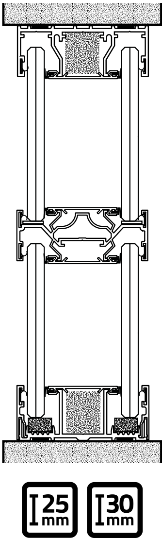
System Silence Loft Vertical
